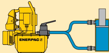
4-way valve used with double-acting cylinder
